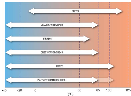
Operating Temperature
