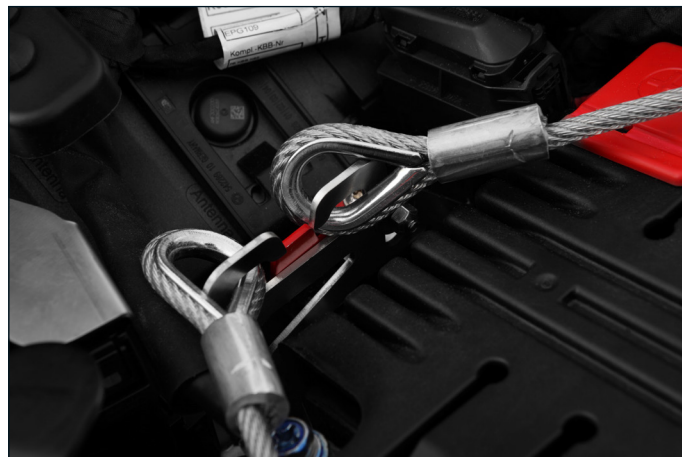
The neatly designed thimbles of the rope ends are hooked into the mounting device of the holding base and securely fixed by a spring-supported latch
