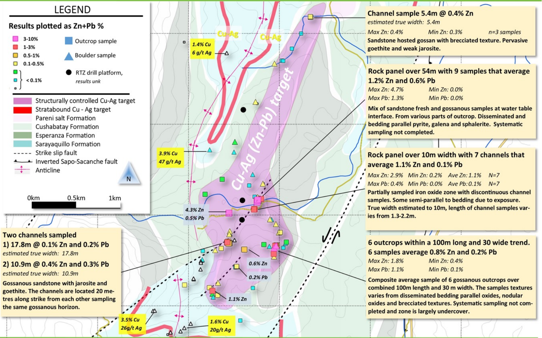
Figure 3. Summary of zinc-lead results from South Sacanche (stratabound reduced facies Cu-Ag samples in yellow). RTZ drill platforms have been located and GPS measured by Hannan in the field.
