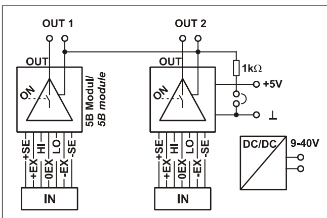
Functional diagram
