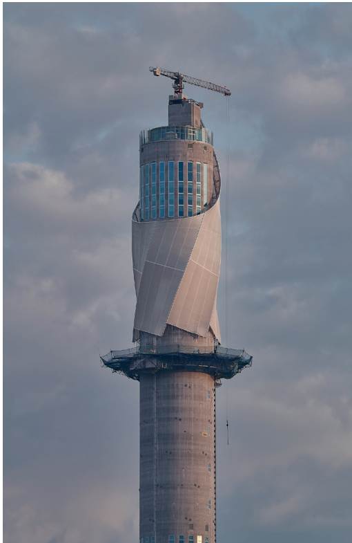
The ThyssenKrupp elevator Test Tower in Rottweil, Germany, photographed during the complicated phase of membrane installation. The facade construction, made from delicate fiberglass mesh developed by Werner Sobek, is currently the world's highest membrane project. Foto: Zoey Braun
