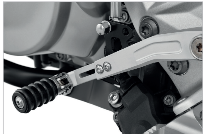
Optically & functionally a highlight: Adjustable gear shift lever on Wunderlich BMW F 750 GS
