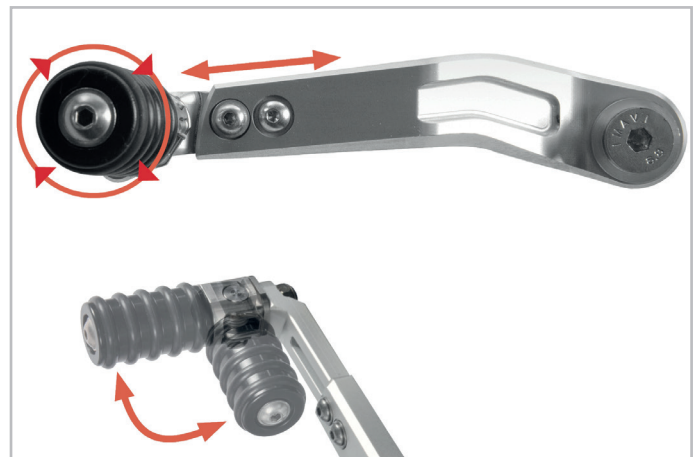
Application example: The »CLEVER LEVER« can not only be adjusted in the length but also offers a roller bearing for the highest comfort of shifting possible – Moreover, the lever is foldable up to 90 degrees to prevent itself against any damage.
