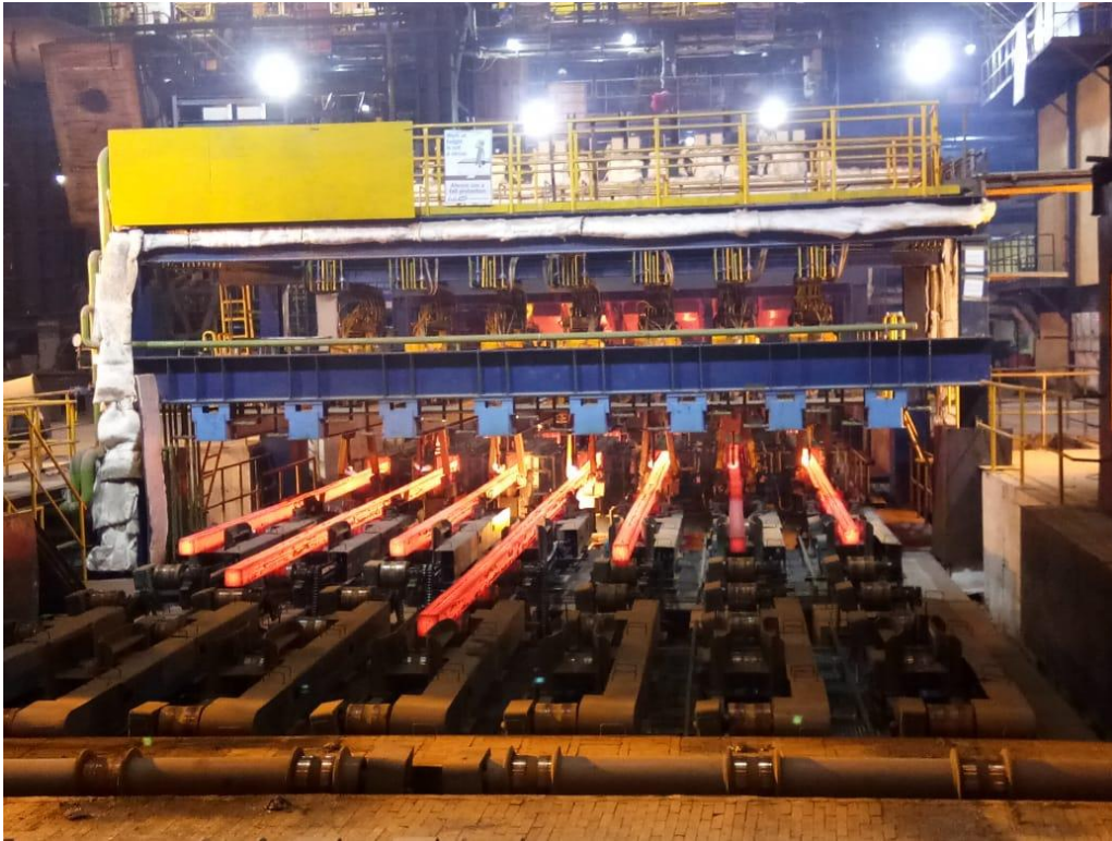
High-speed seven-strand combi-caster in operation at JSPL Angul, India.
