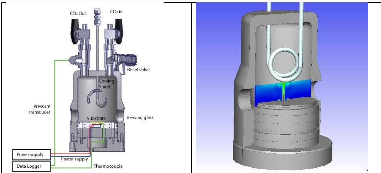
Image: Test facility used by the Danish Technical Institute to measure improved heat transfer of nanostructured substrates (left); corresponding simulation results obtained from ACE+ Suite (right).
